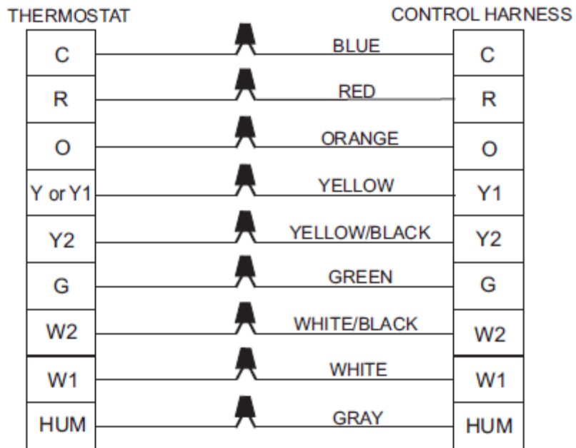
FIGURE 6: Typical Field Control Wiring Diagram For Dual Fuel Models
